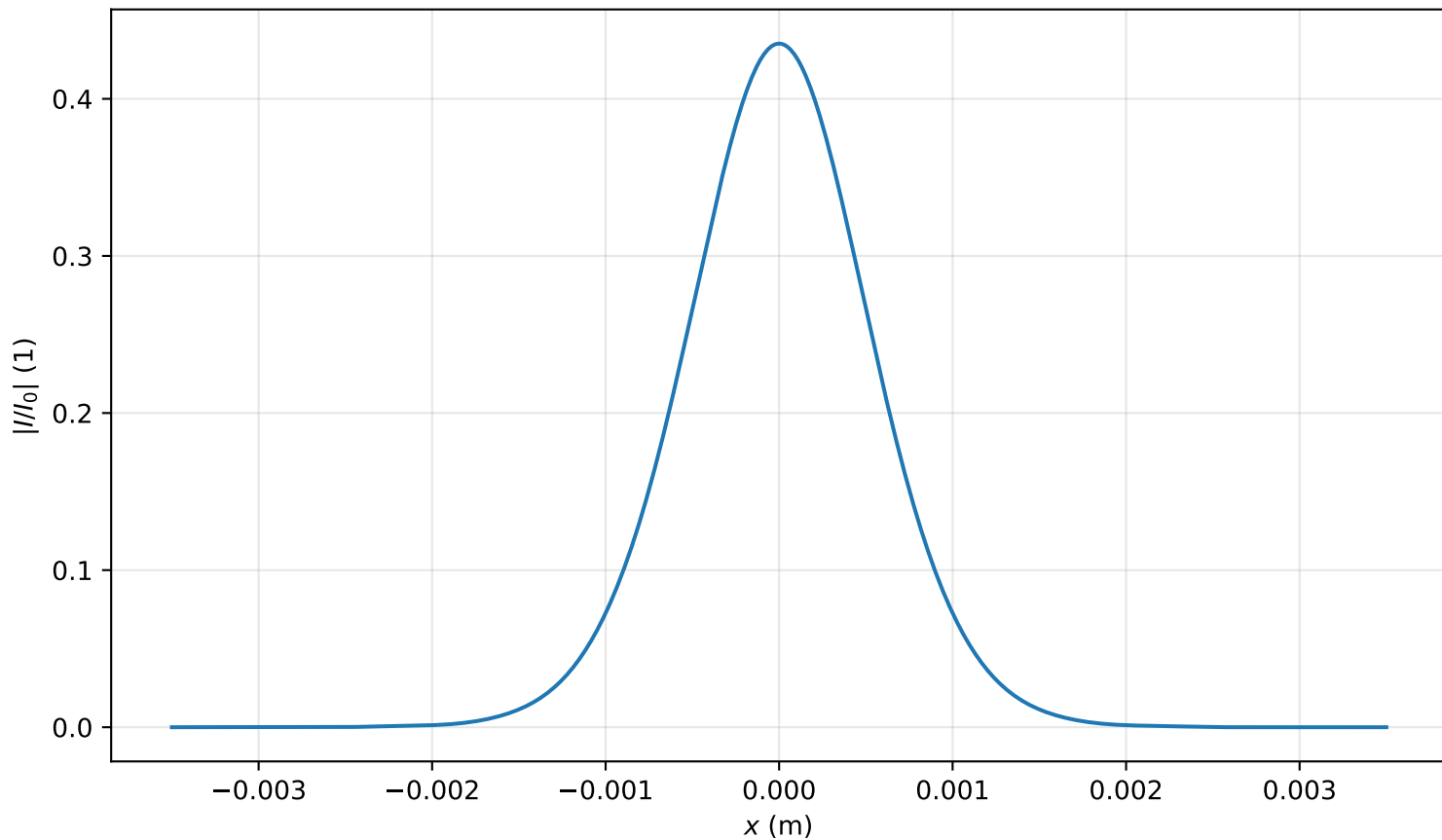
Intensity profile I(x, y = 0, z = 3.264m)/I_0 , P_{in}=0.4P_{cr} , artificial time
